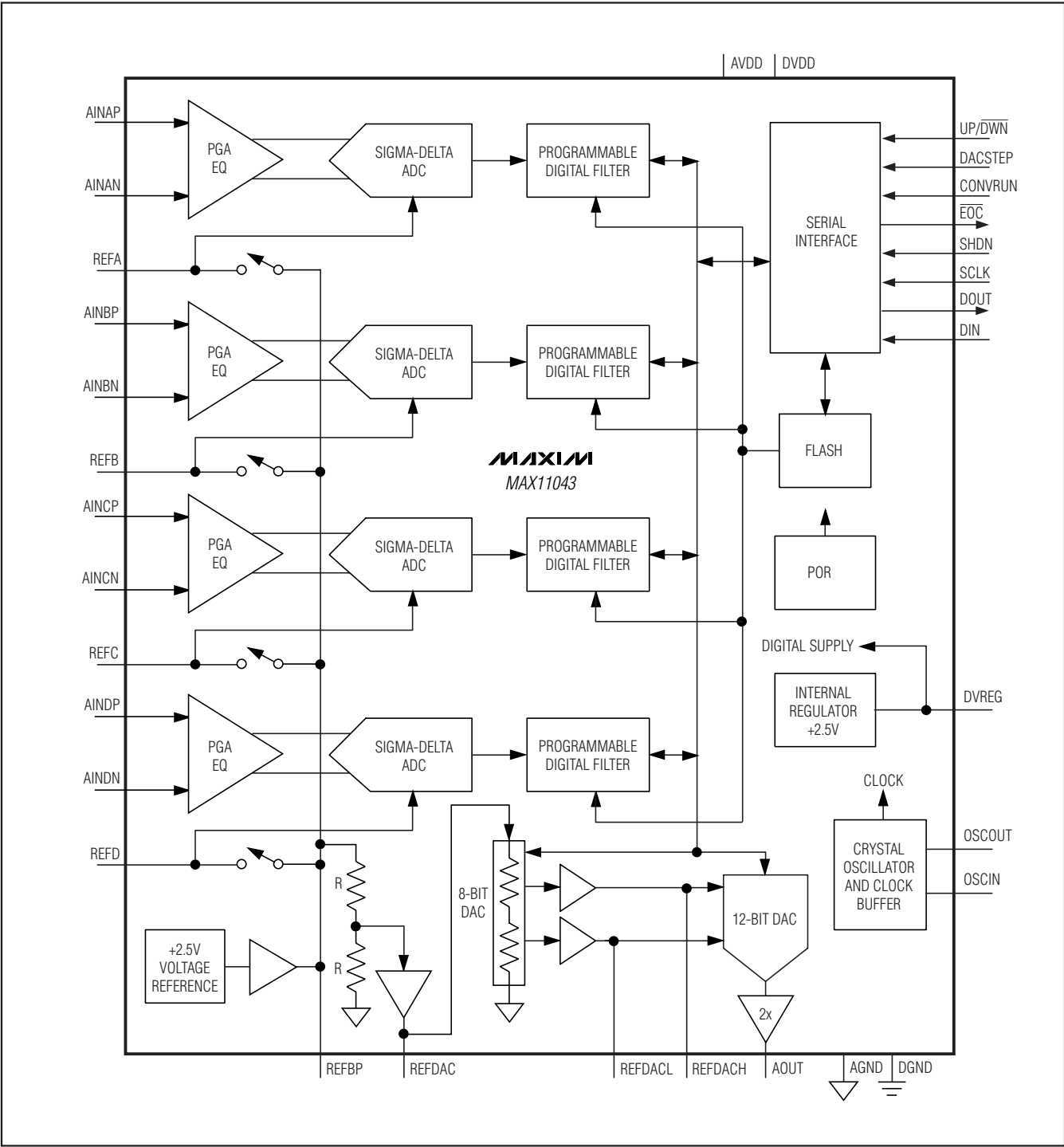
Functional Diagram
